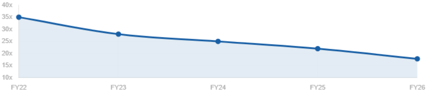
Historical P/E trend (FY22–FY26)
